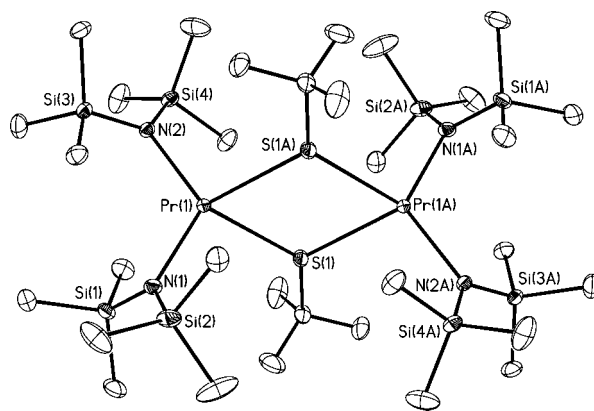
Figure 1. Perspective view of 3 with labelling scheme and 50% thermal ellipsoids. All hydrogen atoms are omitted for clarity.
